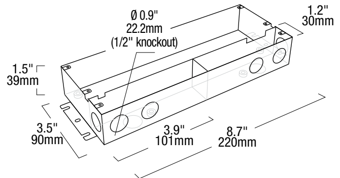
JUNCTION BOX
